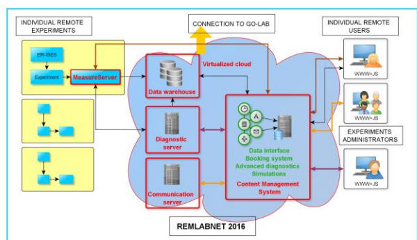
Figure 1 – block diagram of REMLABNET
